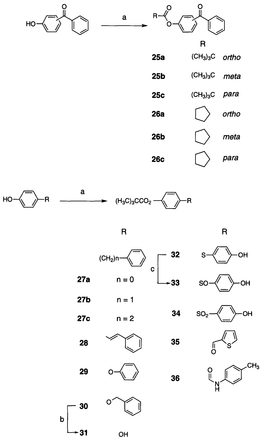
Scheme 3. (1) Preparation of 25a–c and 26a–c. Reagents: t RCOCl, Et 3 N, CH 2 Cl 2 . (2) Preparation of 27–36. Reagents: t (CH 3 ) 3 CCOCl, Et 3 N, CH 2 Cl 2 , 100% Et 3 N, Et 3 N, 30% H 2 O.
